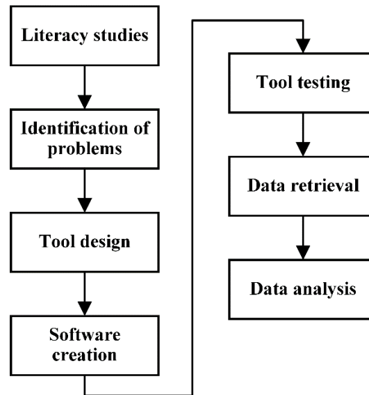
Fig. 4. Research flowchart
