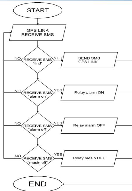
Fig. 2. Flowchart
